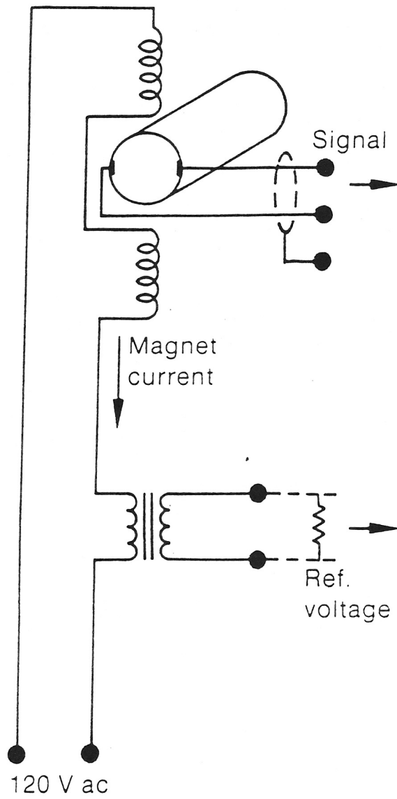
FIGURE 11-2 Typical ac magnetic flowmeter schematic. (Courtesy Fischer & Porter Company)
