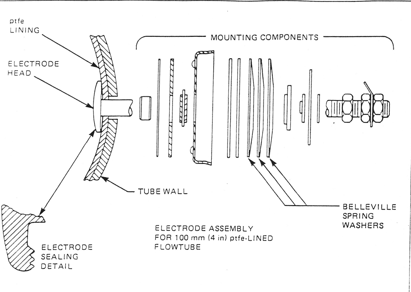
Figure 9-7. Teflon Liner and Electrode
