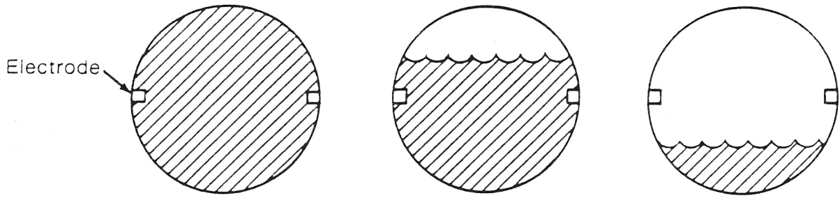
(A) Full pipe: correct
