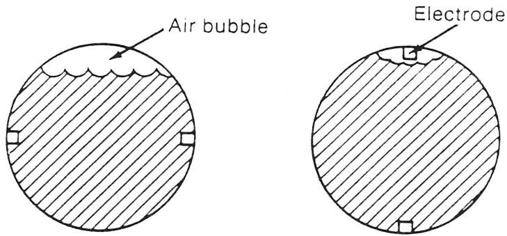
(A) Horizontal orientation: correct
